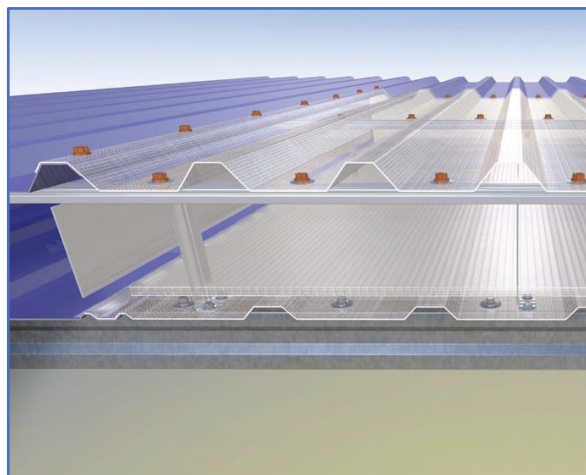
Figure 1.7 – Multi-layered rooflight incorporated into built up roof system
