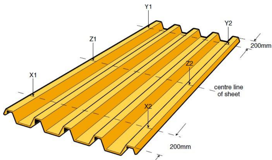
Fig 1: Cover width
