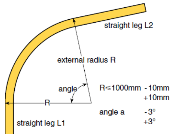
Fig 4: Curve dimensions
