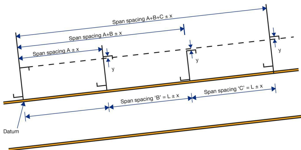
Figure 3 Limits on span position
