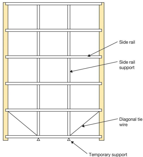
Figure 5 Side rail support during installation
