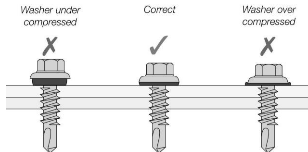
Fig 15: Correct installation for primary fasteners
