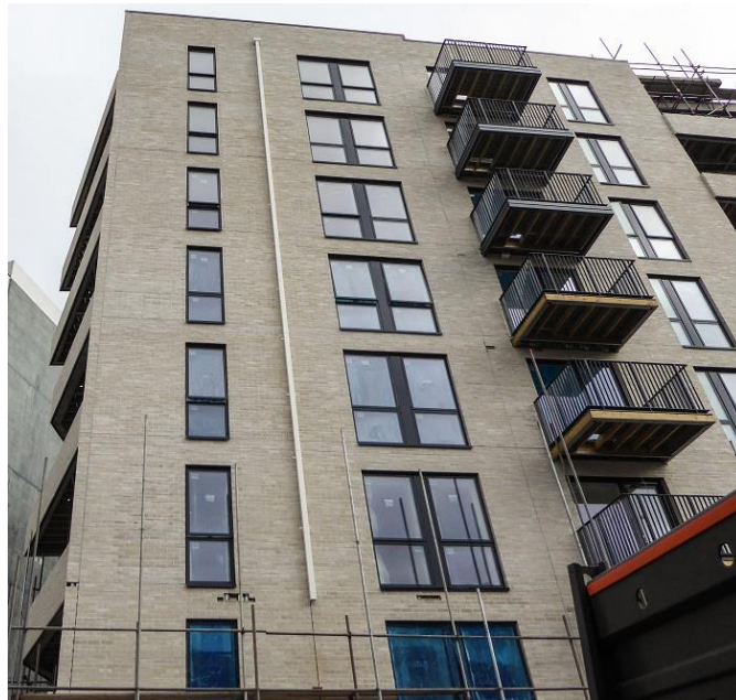
Neat collars of rear fixing pipe clips provide clean lines
