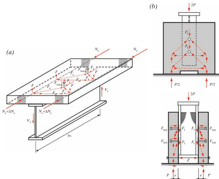
Fig. 1: Internal forces within (a) a composite beam and (b) a push test 1
