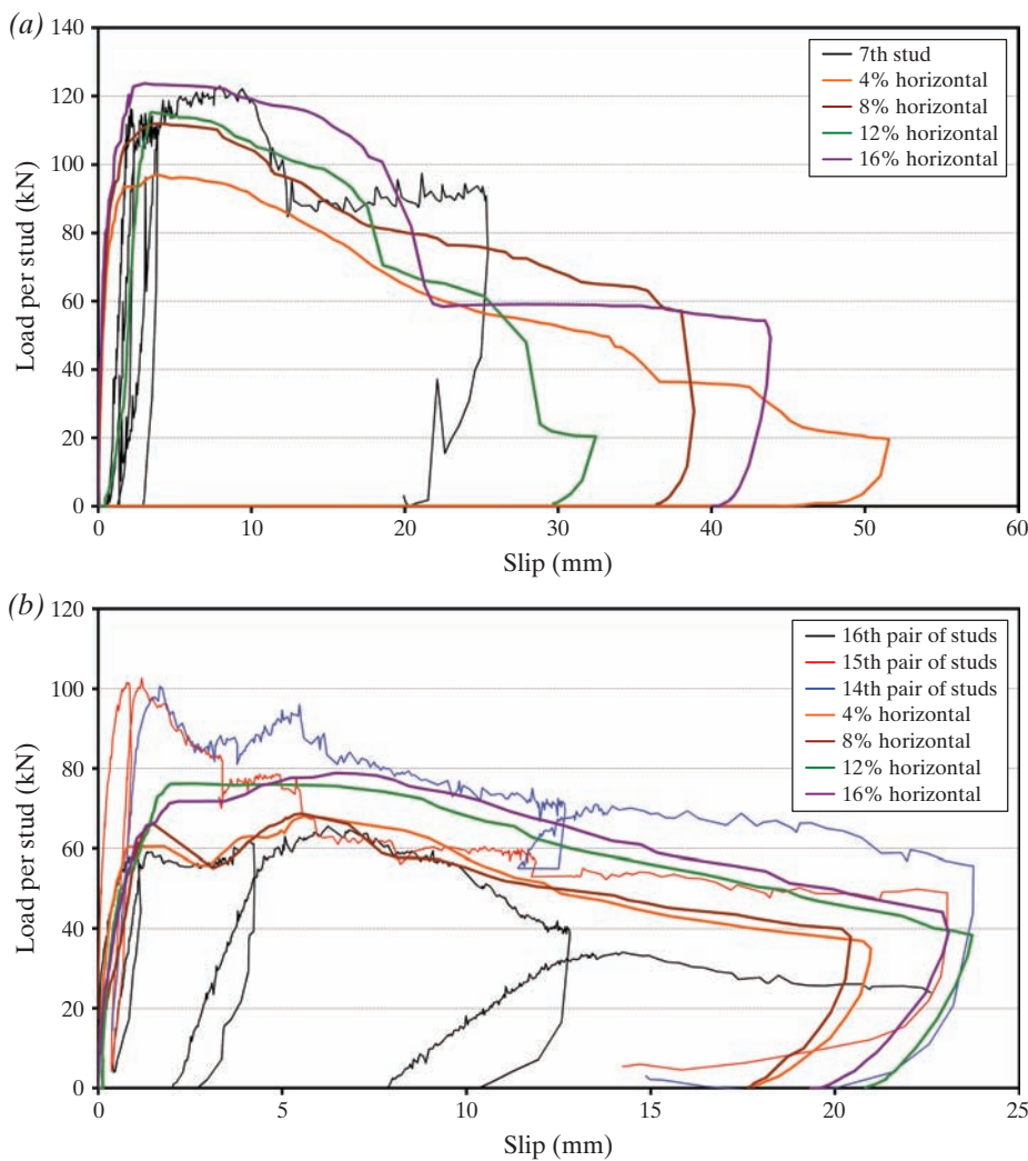
Fig. 6: Comparison of load-slip behaviour for the new improved test with that measured in beam tests for (a) n_r = 1F and (b) n_r = 2F
