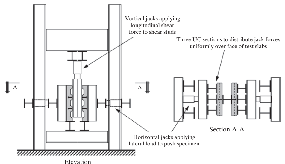
Fig. 5: Improved push test rig
