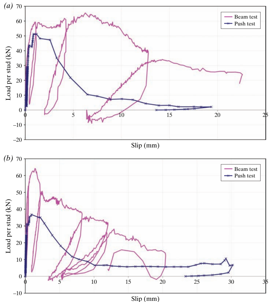
Fig. 4: Load-slip curve for beam test compared to standard push test for (a) n_r = 2F and (b) n_r = 3F
