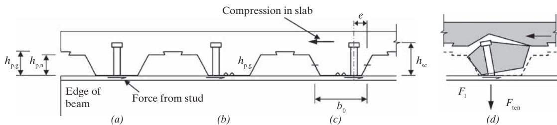
Fig. 2: Dimensions of profiled steel sheeting and studs in the (a) central; (b) favourable; (c) unfavourable position; and (d) concrete pull-out failure
