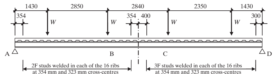
Fig. 3: General arrangement of composite beam test specimen (Units: mm)
