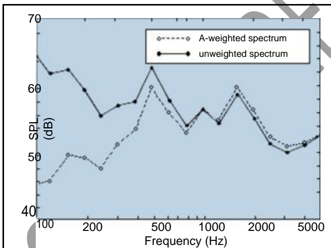
Fig. 3 Typical unweighted and A weighted noise spectra.
