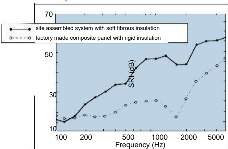
Fig. 12 Comparing a site assembled system and a composite panel.
