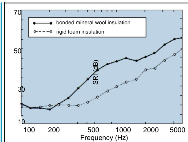
Fig. 13 Comparing site assembled systems with profiled mineral fibre and profiled rigid foam insulation.
