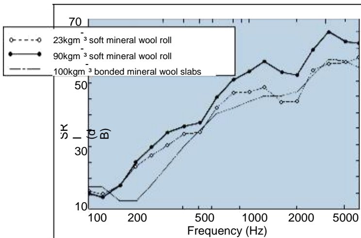
Fig. 11 Comparing the effect of density and softness of mineral fibre insulation
