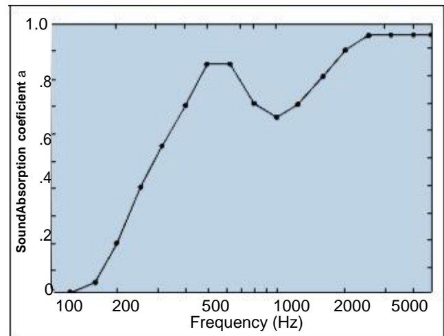
Fig. 4 Acoustic absorption coefficient for a typical fibrous material.
