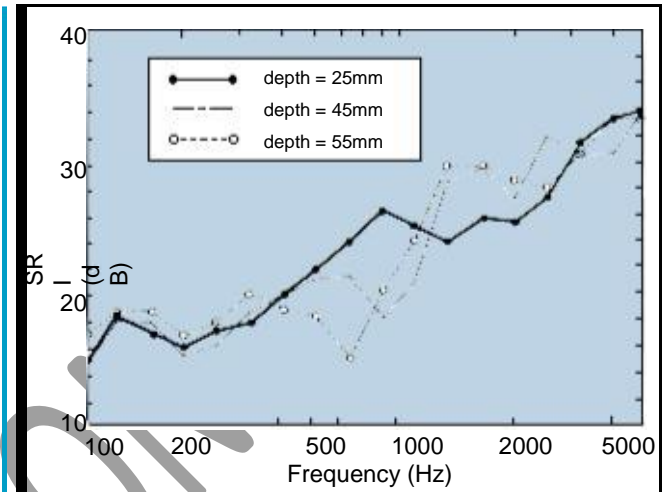
Fig. 7 Effect of profile depth
