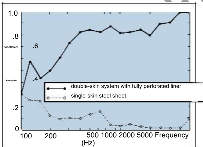
Fig. 14 Comparing sound absorption coefficients of a single skin cladding and a double skin system with perforated liner.
