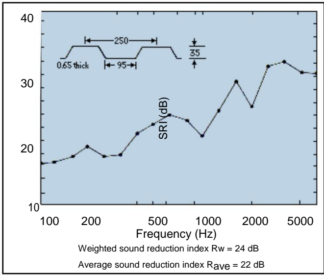
Fig 5 Sound reduction of a profiled metal sheet
