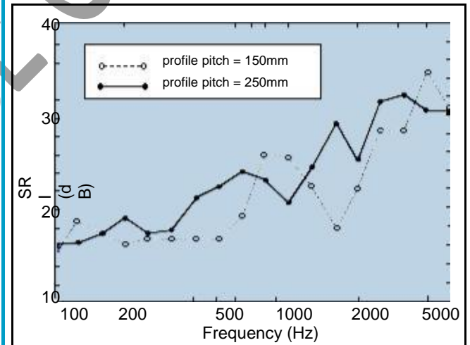
Fig. 8 Effect of profile pitch
