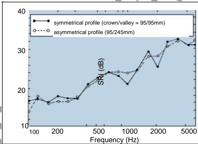
Fig. 6 Effect of profile shape or symmetry
