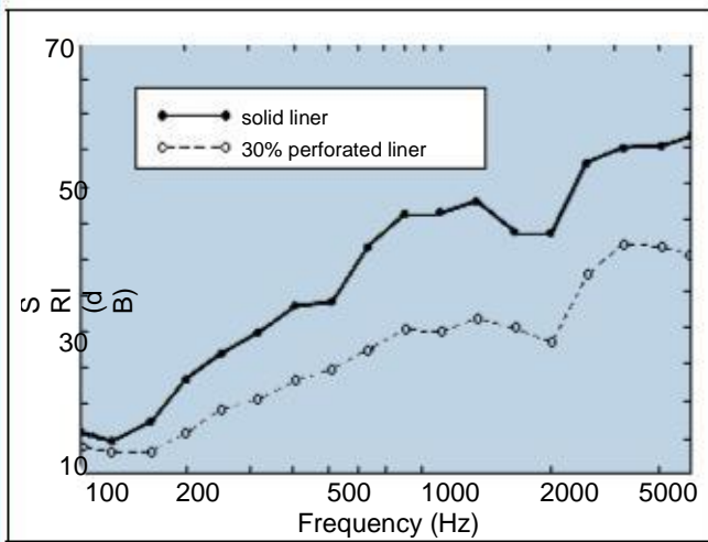
Fig. 15 Effect of perforated liner on sound insulation of a double skin system.
