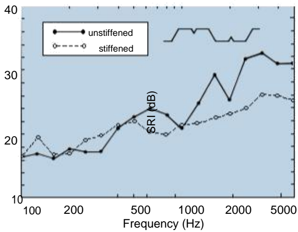
Fig. 10 Effect of stiffeners
