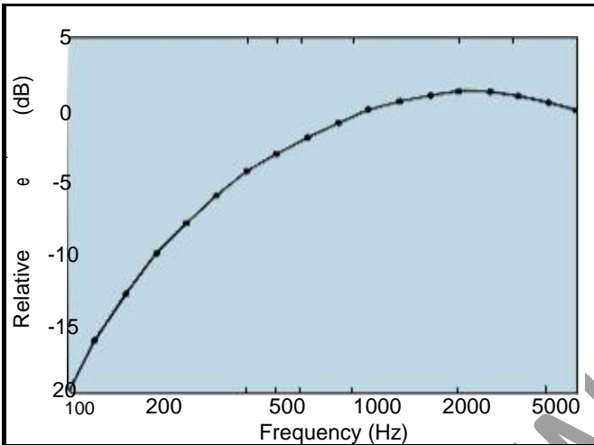
Fig. 2 The A weighting curve
