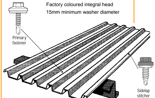
Fig 18: Single skin construction
