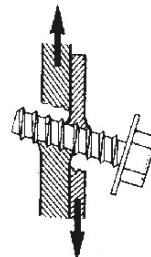
Fig 15: Shear load resistance
