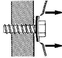
Fig 14: Pullover resistance
