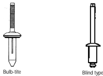
Fig 5: Rivet type fasteners
