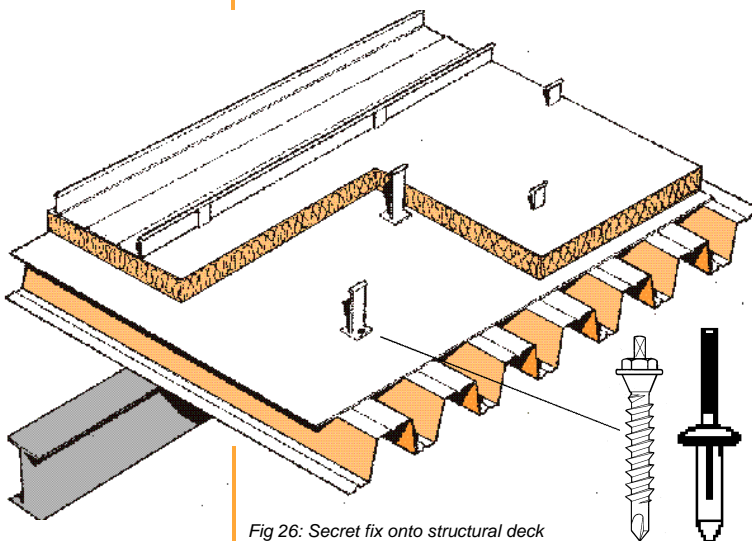
Fig 26: Secret fix onto structural deck
