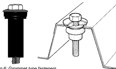
Fig 6: Grommet type fasteners
