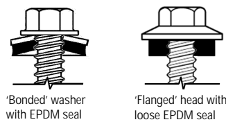
Fig 10: Washer types
