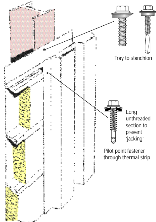
Fig 27: Structural liner tray
