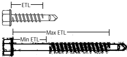
Fig 32: Effective thread length (ETL)
